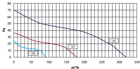
TUBO 100/120/150 TP
