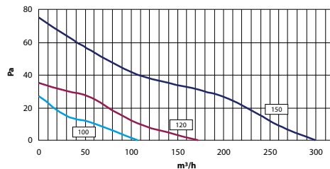
TUBO 100/120/150 METAL
